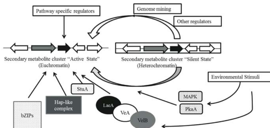
Fig. 1. Regulation of fungal secondary metabolism by transcriptional regulatory elements. SM gene clusters are often silent in laboratory conditions. Activation of SM clusters is complex and involves several layers of transcriptional regulators from pathway specific regulators to more global regulators such as bZip proteins, StuA and Velvet (LaeA, VeA, and VelB) and Hap-like complexes. This activation is associated with conversion of heterochromatin marks (silent cluster) to euchromatin marks (active cluster). In addition, environmental stimuli are translated by signal transduction cascades, including MAPK and PkaA, to activate SM synthesis.
